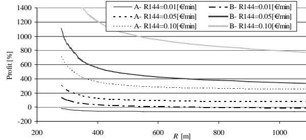
Fig. 10. Profit per \text{km}^2 as a function of R (three amplifiers).
