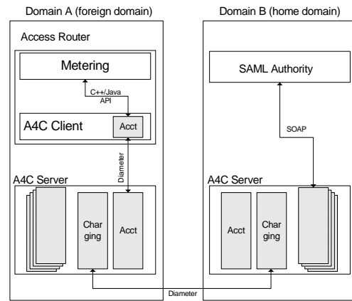
Figure 4: Accounting Implementation Architecture
