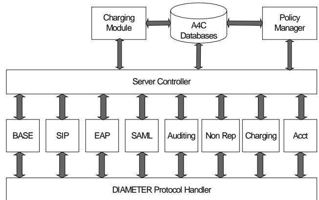
Figure 5: Internal A4C Server Architecture
