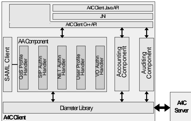
Figure 6: Internal A4C Client Architecture
