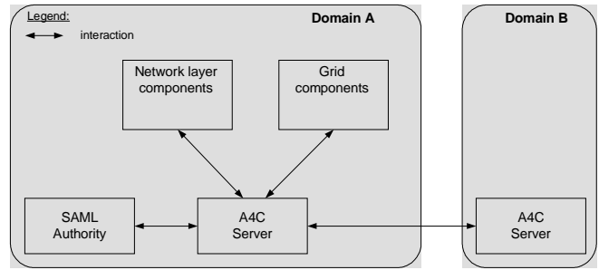
Figure 3: A4C Architecture Components
